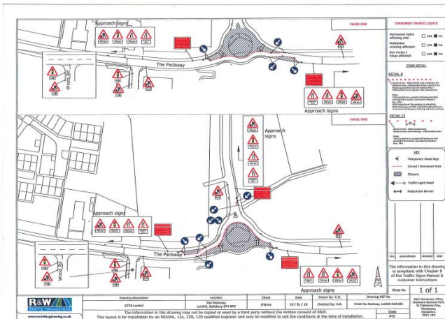
The Packway 4-way gyratory system
